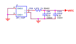
RTC BATT
